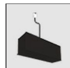
150W Ceiling power supply kit (cable length 2,2 m) - 230VAC- 48VDC - IP20 - 321x91x111H - Black - DALI AQ17704
