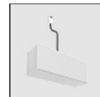
240W Ceiling power supply kit (cable length 2,2 m) - 230VAC-48VDC - IP20 - 321x91x111H - White - DALI AQ17201
