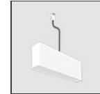
240W Ceiling power supply kit (cable length 2,2 m) - 230VAC-48VDC - IP20 - 321x91x111H - White - Undimmable AQ17301
