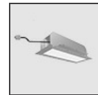
240W Recessed power supply kit (cable length 2,2 m) - 230VAC-48VDC - IP20 - 396x195x112H - DALI AQ16801
