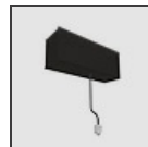
150W Ceiling power supply kit (cable length 2,2 m) - 230VAC-48VDC - IP20 - 321x91x111H - Black - DALI AQ17504
