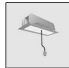
240W Recessed power supply kit (cable length 2,2 m) - 230VAC-48VDC - IP20 - 396x195x112H - White - Undimmable AQ17401
