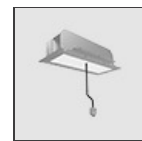
240W Recessed power supply kit (cable length 2,2 m) - 230VAC-48VDC - IP20 - 396x195x112H - White - APP Compatible AQ15401APP
