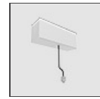
150W Ceiling power supply kit (cable length 2,2 m) - 230VAC- 48VDC - IP20 - 321x91x111H - White - APP Compatible AQ17501APP
