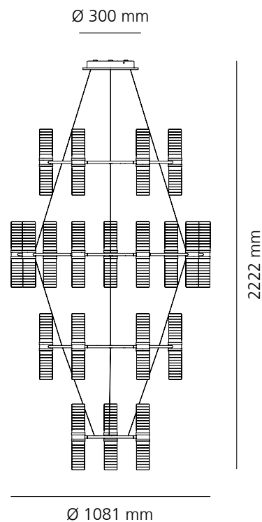
Zephyr Chandelier
