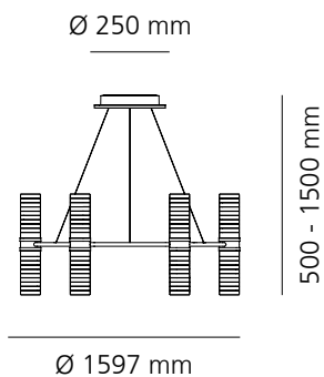
Zephyr R
