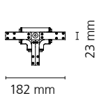
T Joint
