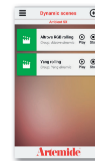
DYNAMIC SCENES
